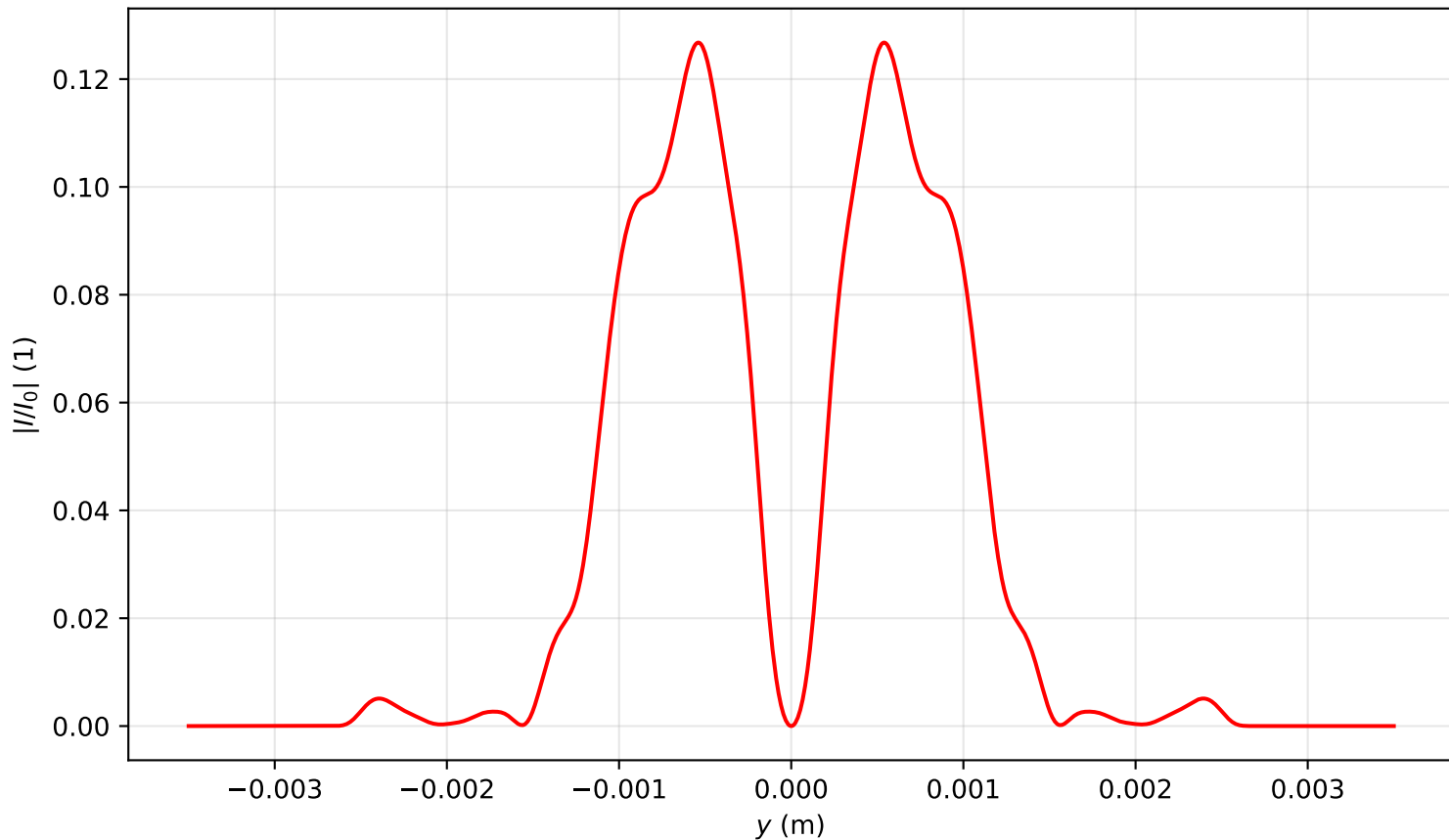
Intensity profile I(x=0, y, z=2.866)/I_0 , P_{in}=7.0P_{cr} , artificial time
